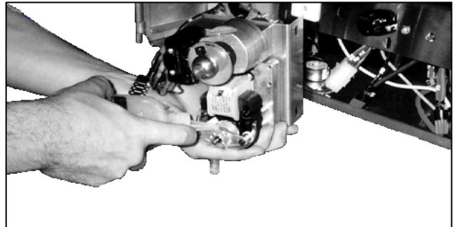
Figure 3-4. Lubricating the Conveyor Drive Motor.
