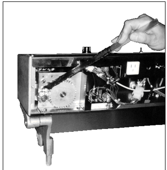
Figure 3-2. Lubricating the Drive Gears.
