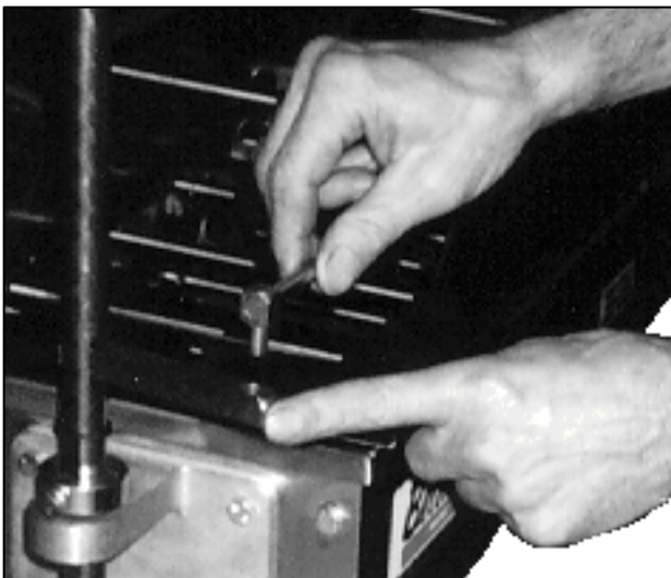
Figure 1-4. Connecting the Swing Connecting Rod.
