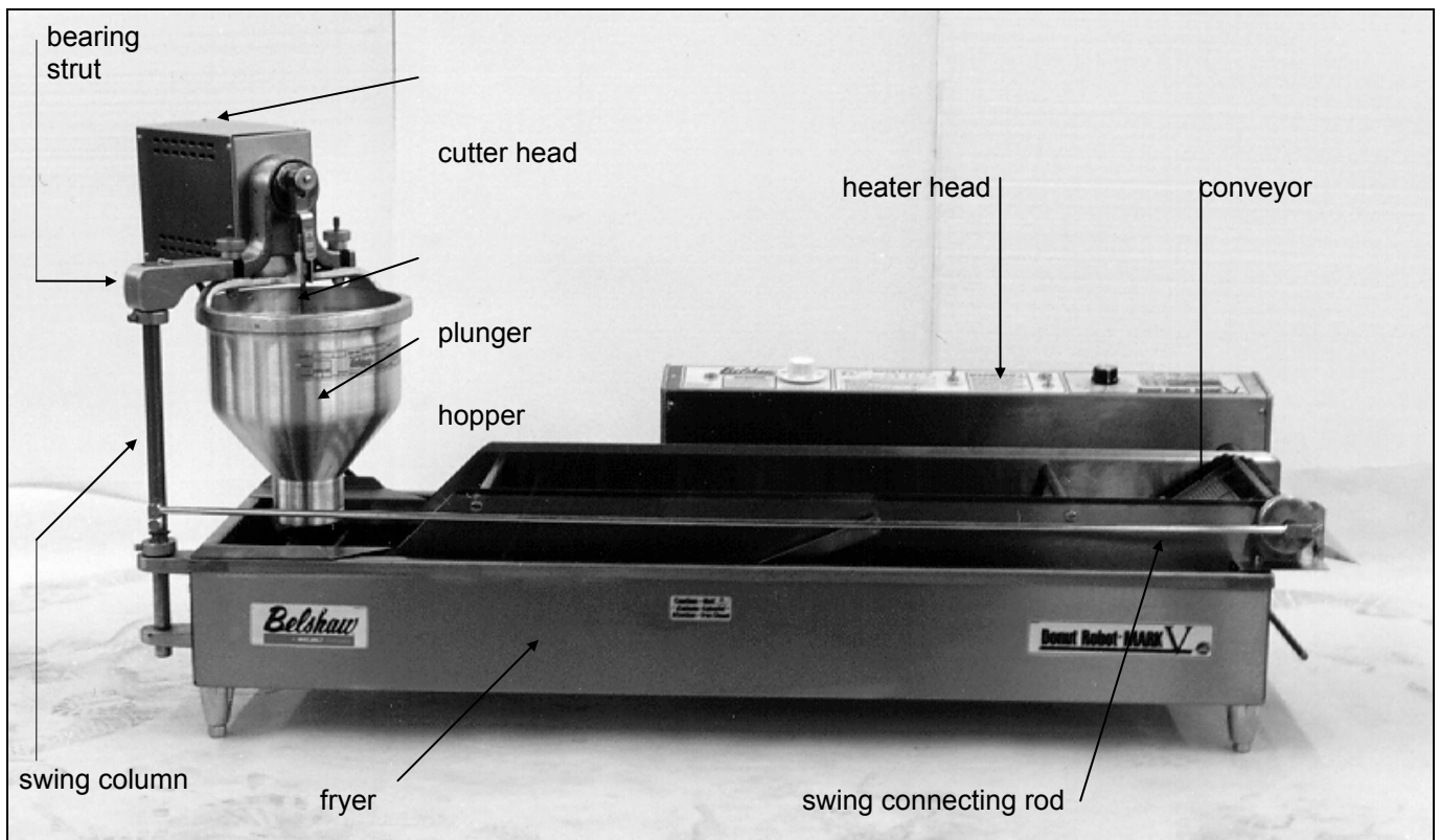
Figure 1-1. Donut Robot Mark V, Front View.
