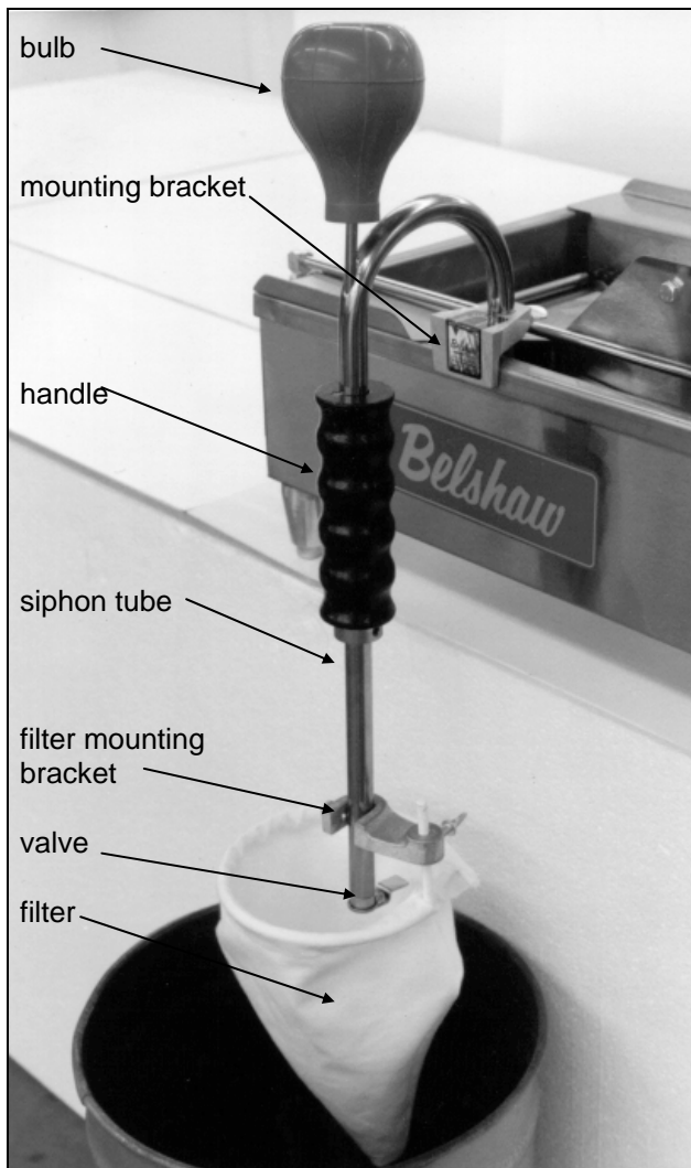
Figure 4-5. Filter Flo Siphon.
