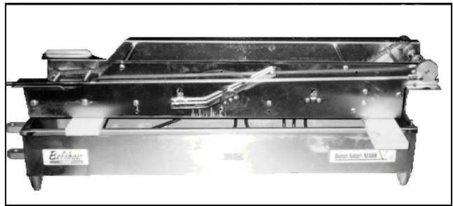
Figure 2-1. Draining the Shortening off of the Conveyor.
