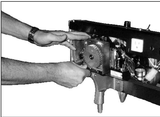
Figure 3-3. Removing the Conveyor Drive Motor.
