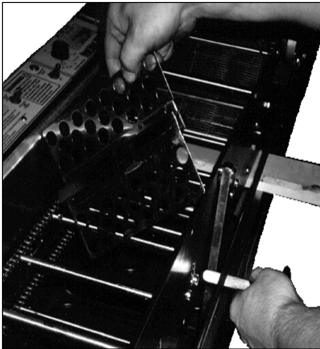
Figure 2-3. Removing the Turner Assembly.
