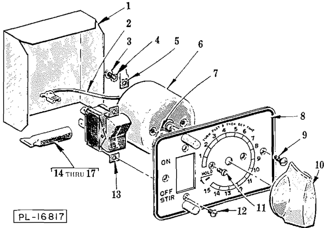
SWITCH & TIMER UNIT (AS200) (MACHINE ML'S, 19208, 19220, 19222 & 19224)
