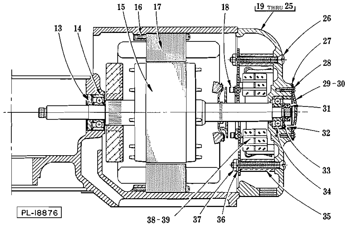
MOTOR PARTS (AS200 SERIES) (SEE PAGE 10 FOR A200 SERIES)
