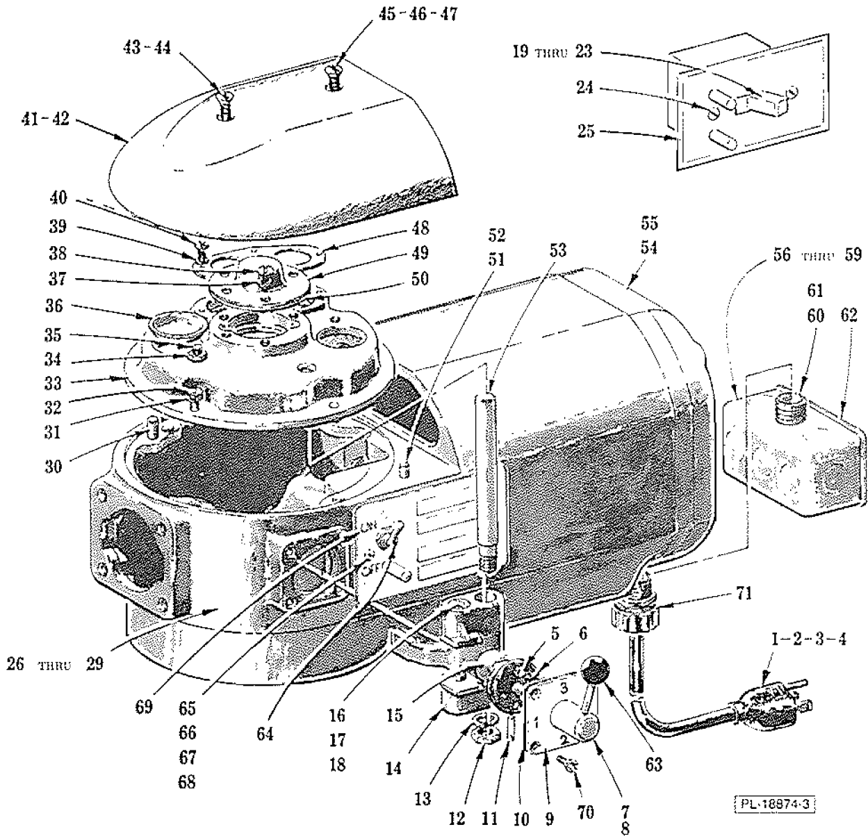
TRANSMISSION CASE & SHIFTER UNIT (A200 SERIES) (SEE PAGE 12 FOR AS200 SERIES)
