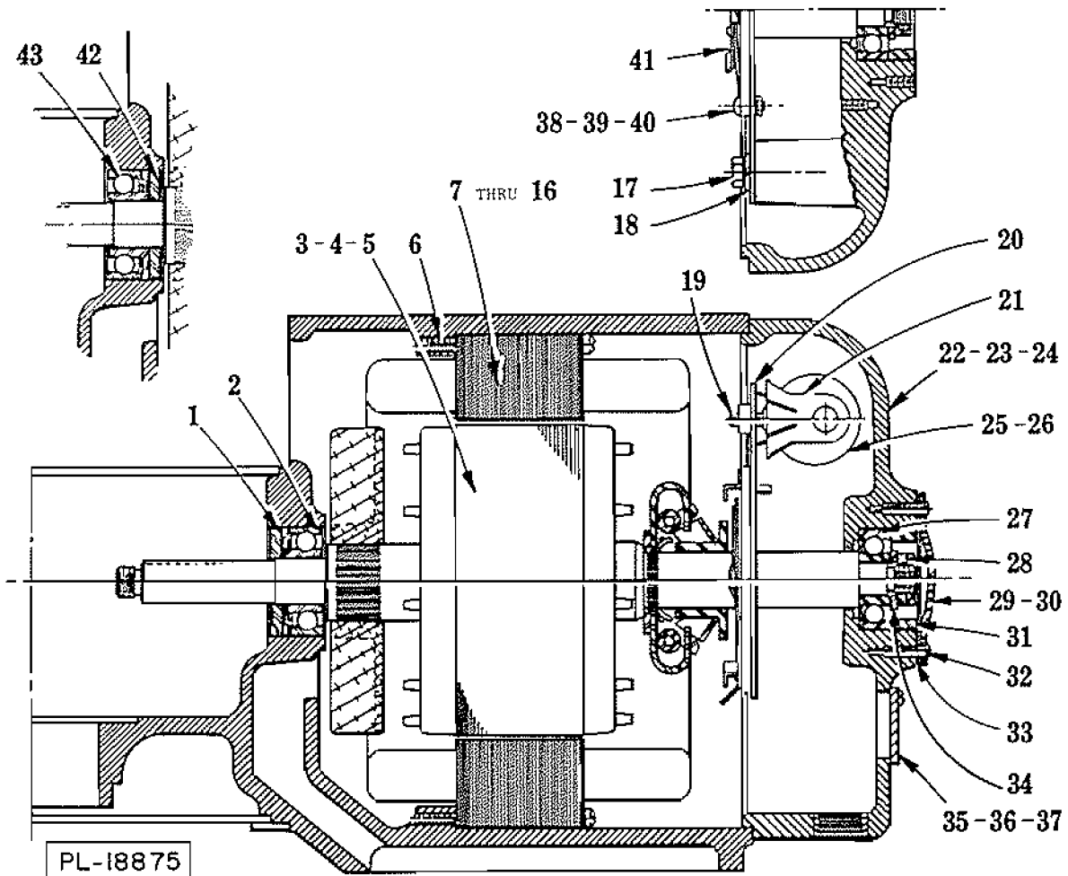
MOTOR PARTS (A200 SERIES) (SEE PAGE 14 FOR AS200 SERIES)
