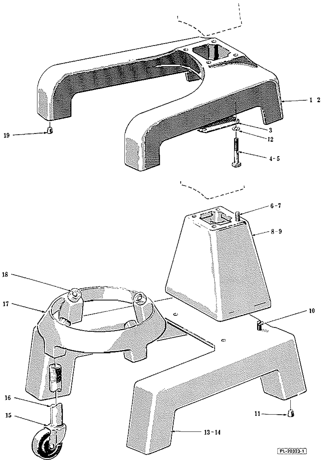
BASE UNIT
