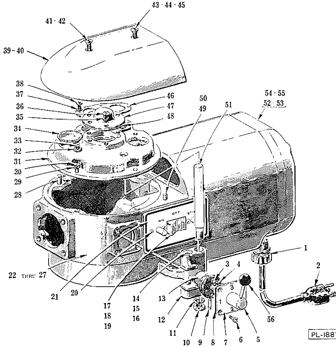
TRANSMISSION CASE & SHIFTER UNIT (AS200 SERIES) (SEE PAGE 8 FOR A200 SERIES)
