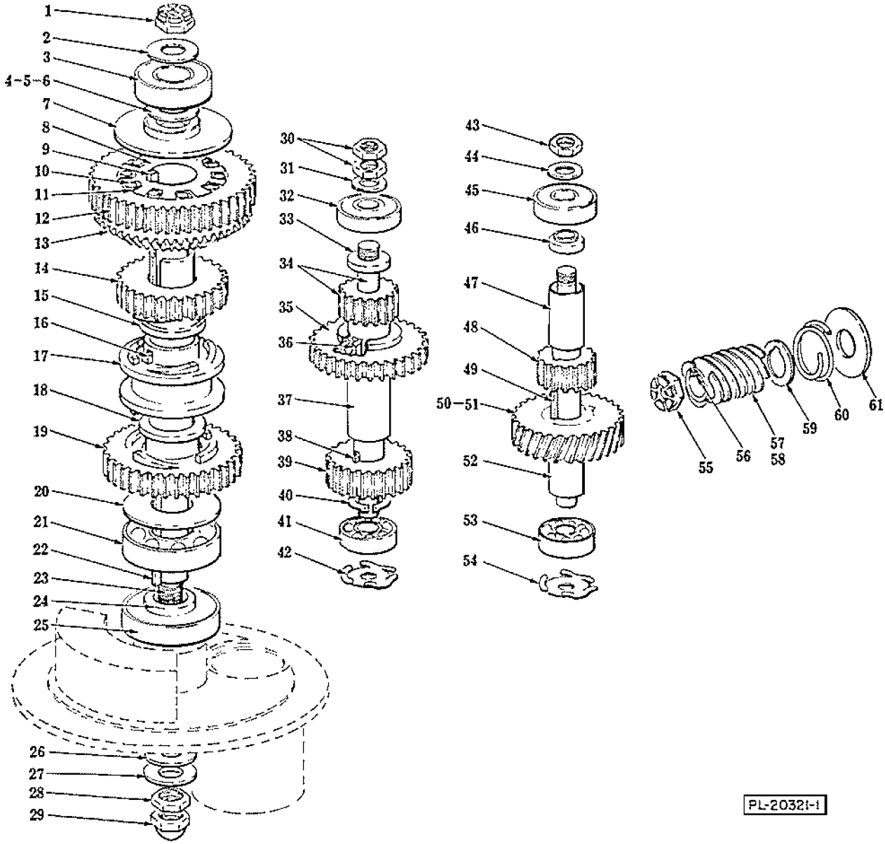
TRANSMISSION GEAR UNIT (MACH. ML-38713 THRU 38729)
