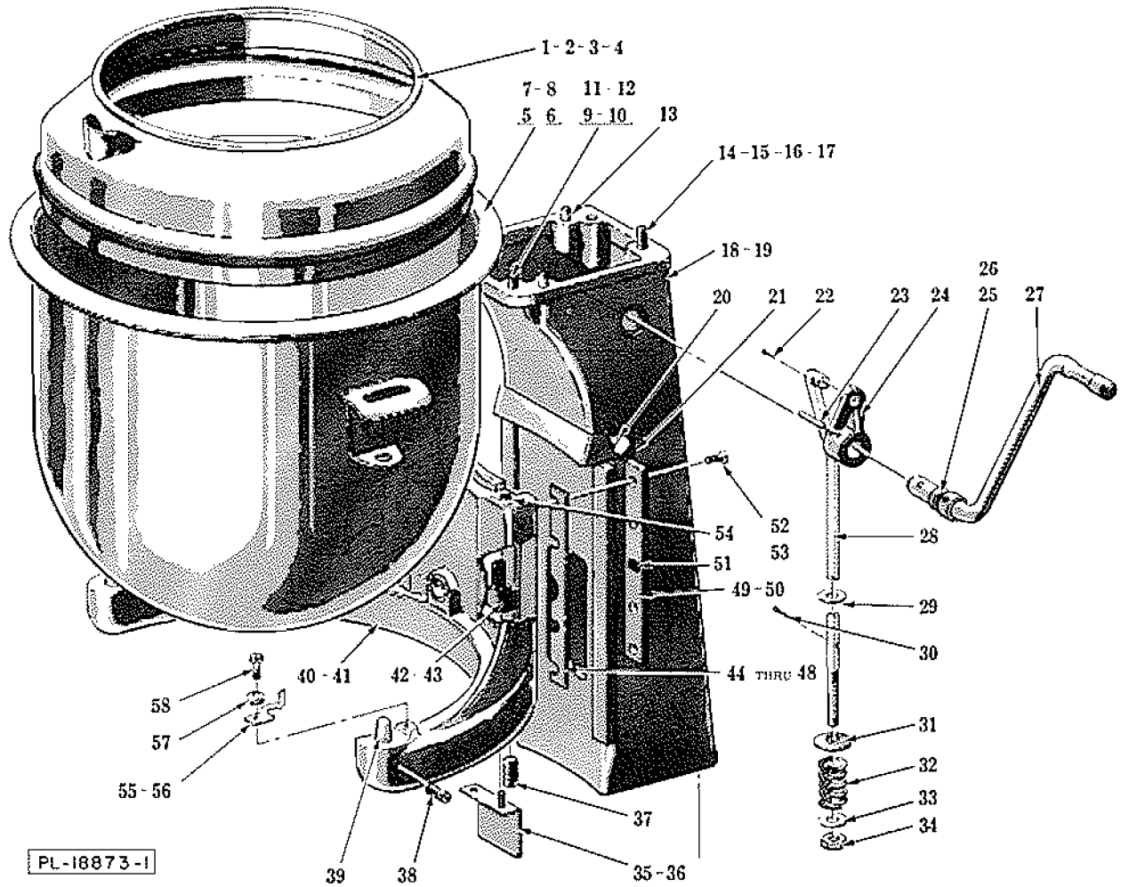
PEDESTAL & BOWL UNIT
