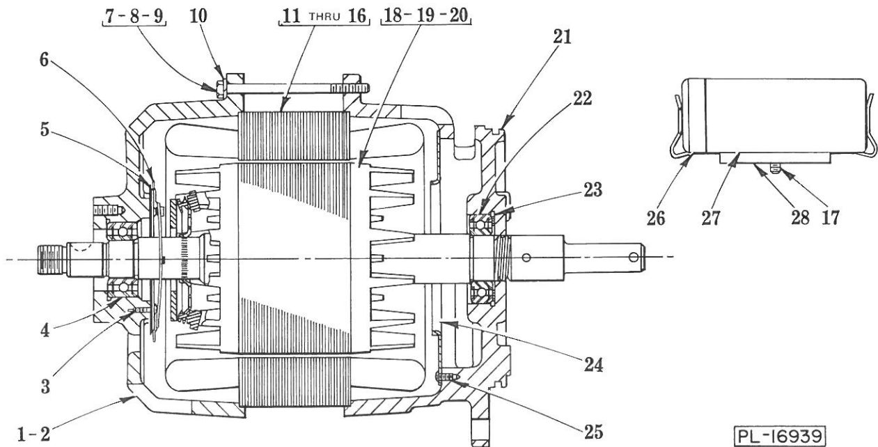
MOTOR UNIT
